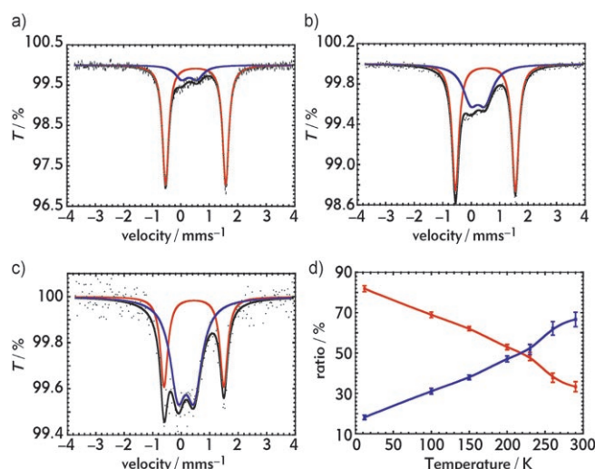
Figure 4. 57 Fe Mössbauer spectra of 5 at a) 12, b) 150, and c) 290 K (see text for explanation of colors), and d) the change in \varphi^{\text{II}} (red) and \varphi^{\text{III}} (blue) as a function of temperature.
